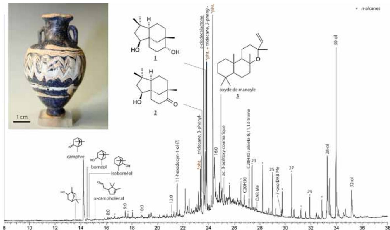
Figure 3 : Chromatogramme de l'extrait lipidique brut (Nora-93). Figure 3: Chromatogram of the total lipid extract (Nora - 93).
